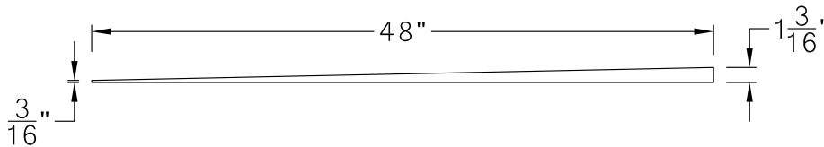
Quick Slope ADA Dimensions
